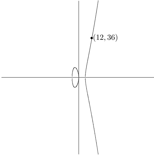
Figure 6.2: The rational point (12, 36) on y^2 = x^3 - 36x .
