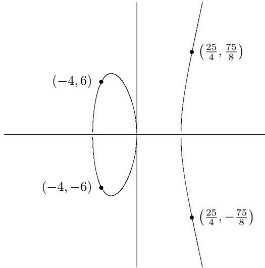
Figure 6.3: Some rational points on y^2 = x^3 - 25x .
